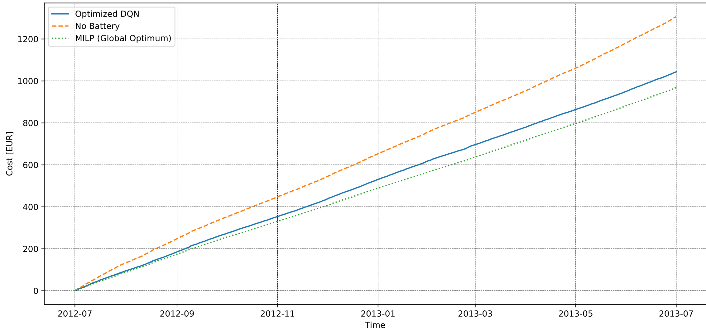
User 128 - Extended Convergence - Electricity Cost [DQN vs MILP]
